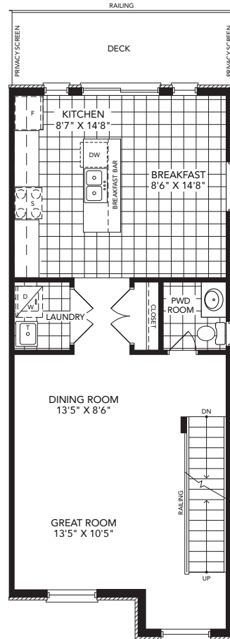
SECOND FLOOR EL-A
