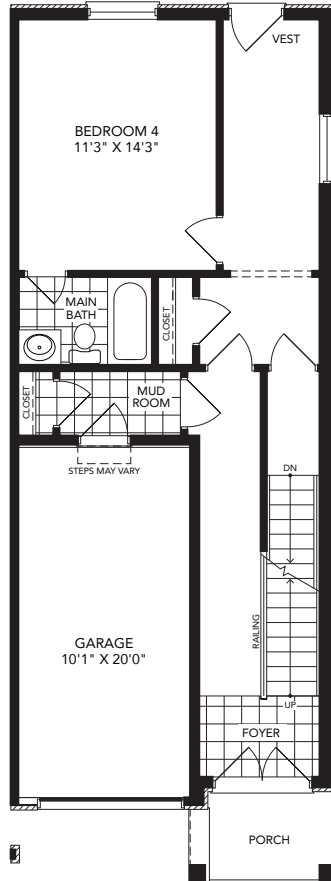
GROUND FLOOR EL-A
